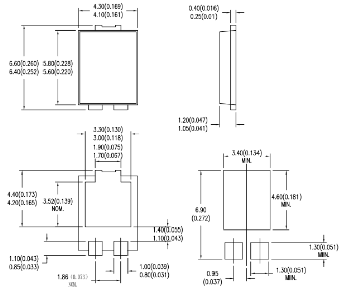
TO-277B
